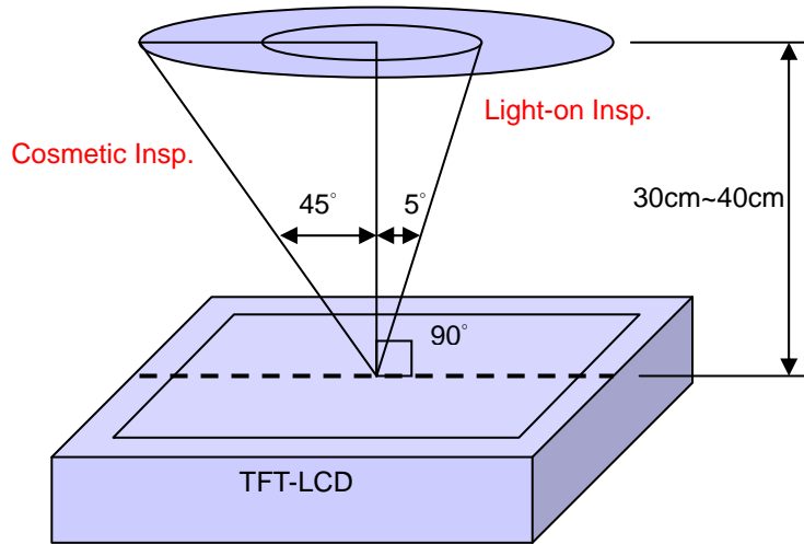
( perpendicular to LCD panel surface)
