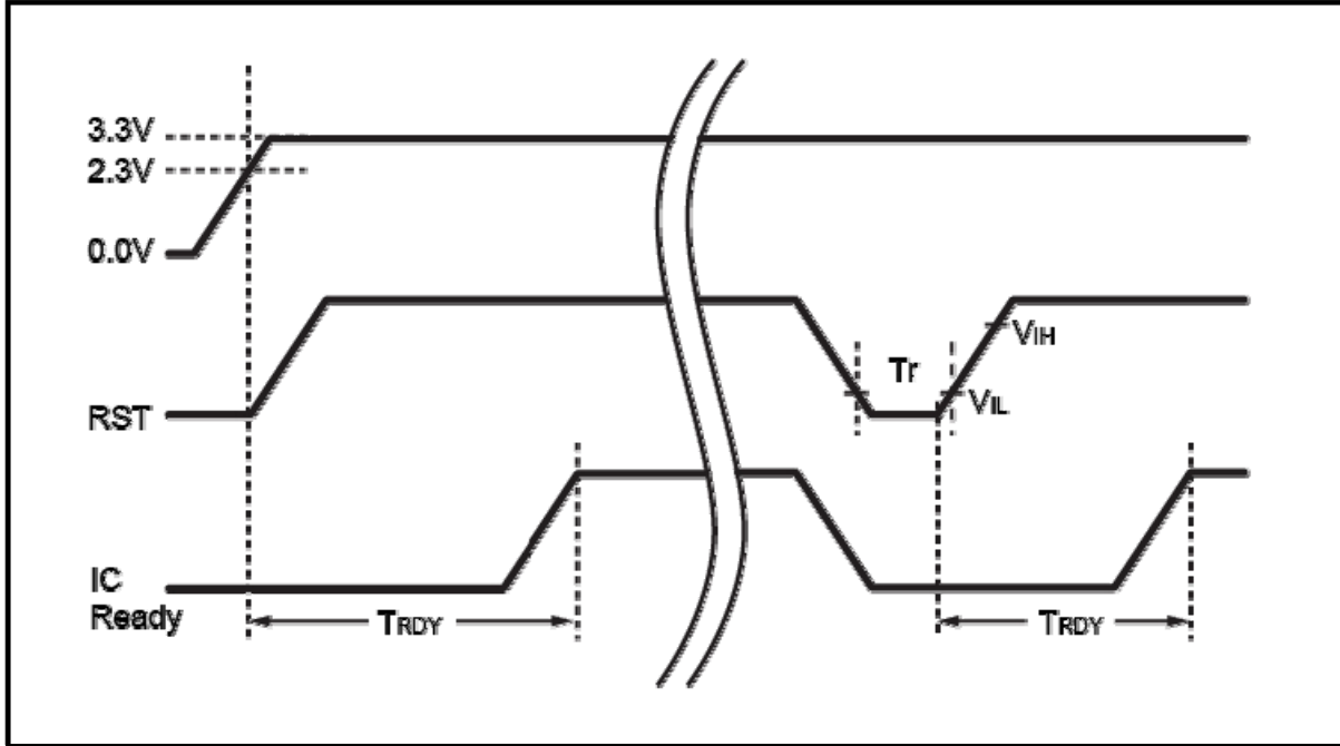
Power On Sequence Diagram
