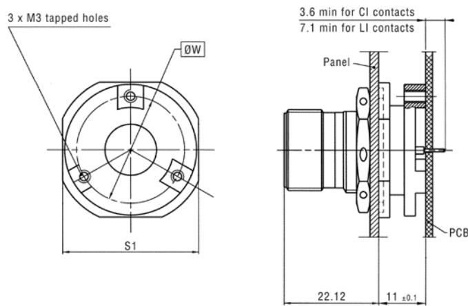
Jam nut receptacle (size 9 and 11)
