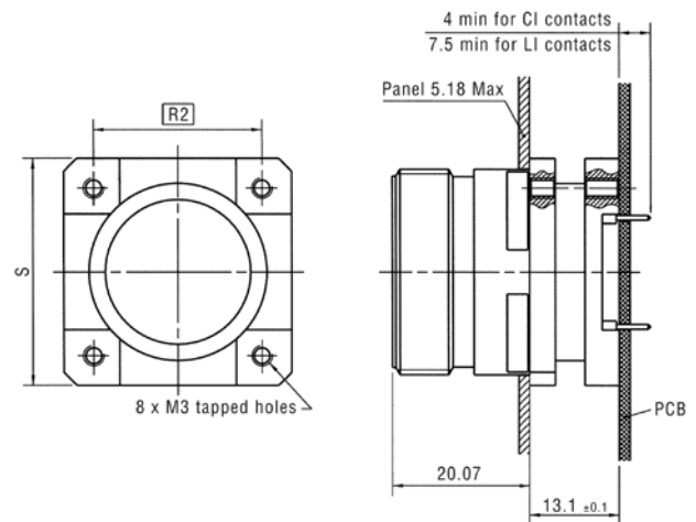
Square flange receptacle (size 9 to 25)
