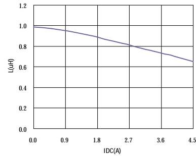
DP25121R5ML□
