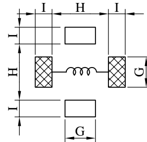
( PCB Pattern )
