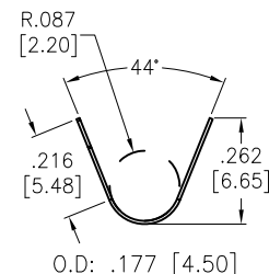
USB-C31-PLUG-B-L1-BK-PCB
